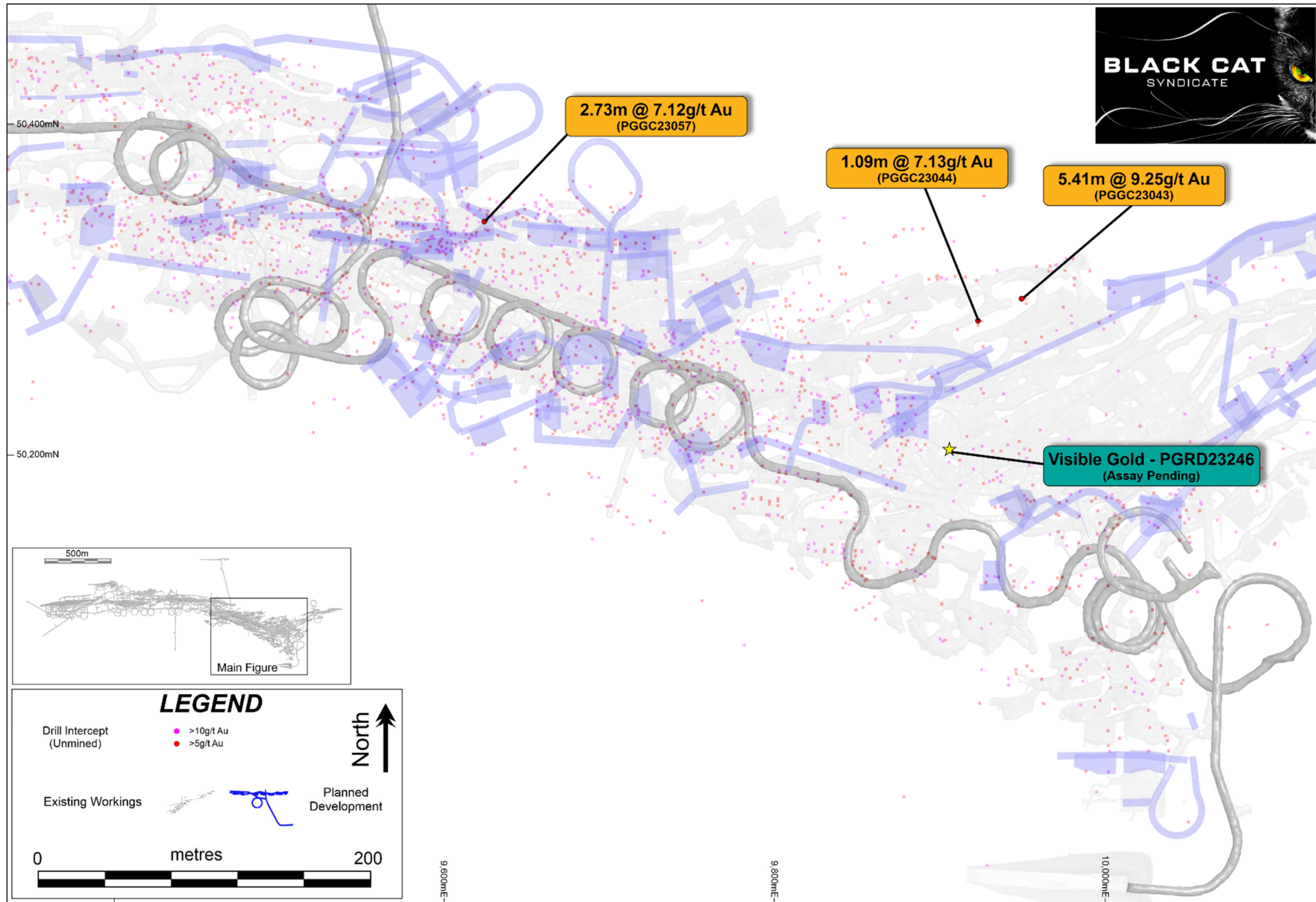
Figure 4: Plan view of the upper section of the mine showing recent drill results from within the Main Zone. Recent results are highlighted. Also shown is the significant quantity of unmined drilling intercepts >5g/t Au (red) and >10g/t Au (purple).
