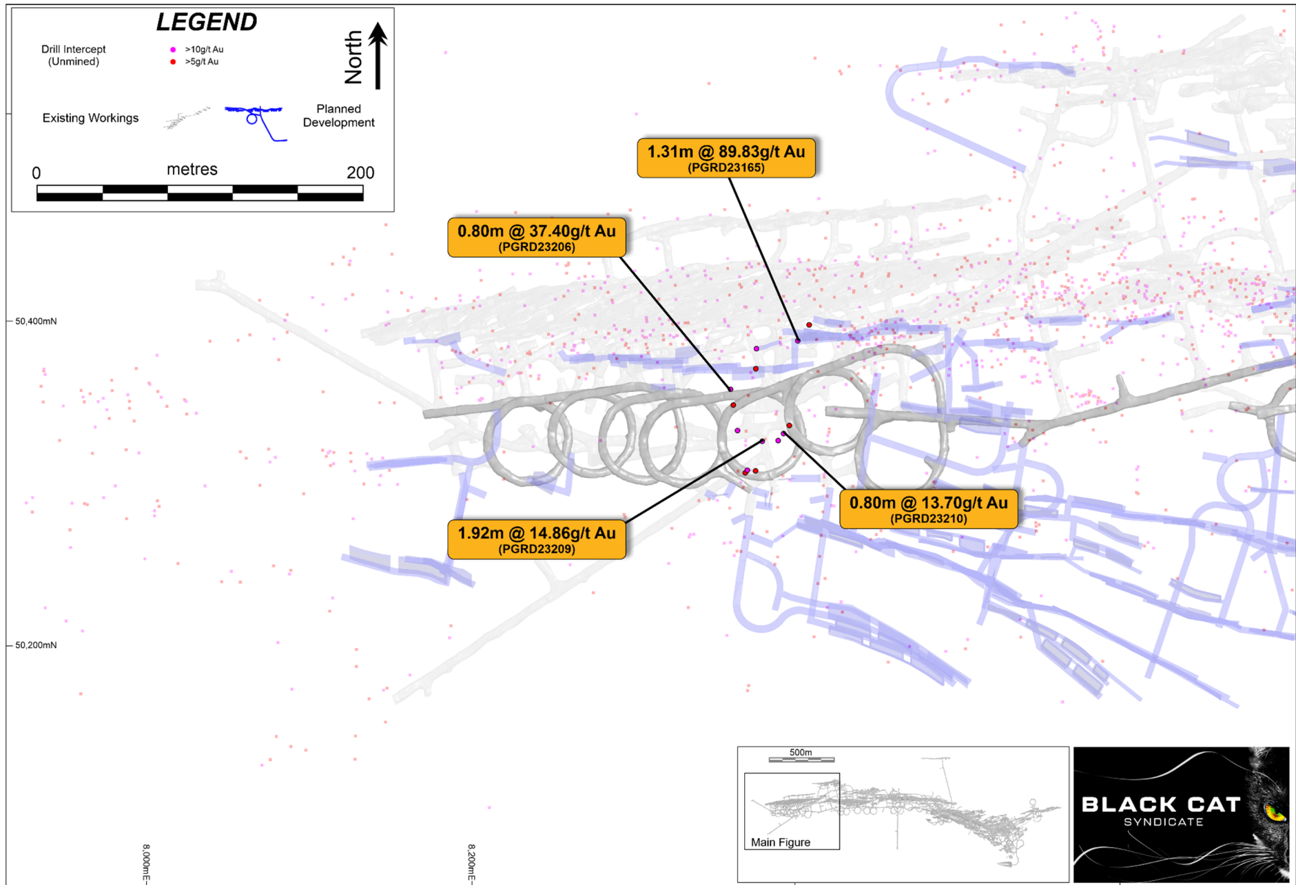
Figure 6: Plan view of the lower section of the mine showing recent drill results from within the Main Zone. Recent results are highlighted. Also shown is the significant quantity of unmined drilling intercepts >5g/t Au (red) and >10g/t Au (purple).
