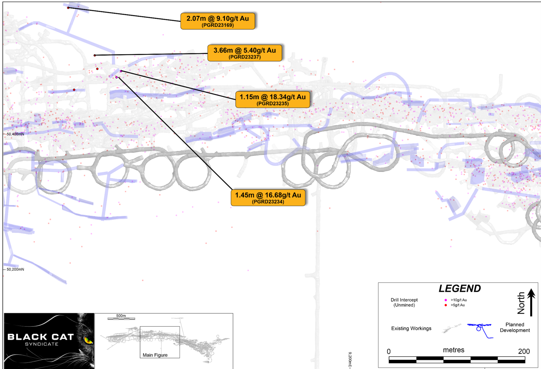
Figure 4: Plan view of the middle section of the mine showing recent drill results from within the Main Zone. Recent results are highlighted. Also shown is the significant quantity of unmined drilling intercepts >5g/t Au (red) and >10g/t Au (purple).
