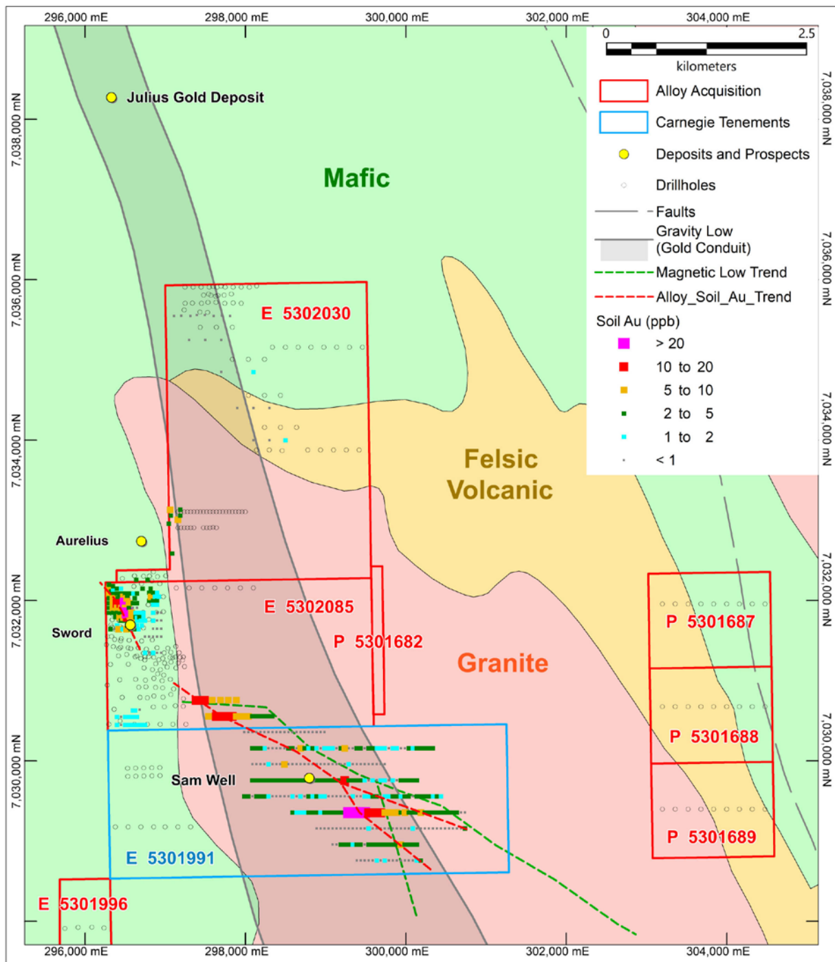
Figure 4. Bronzewing North Geology Interpretation
