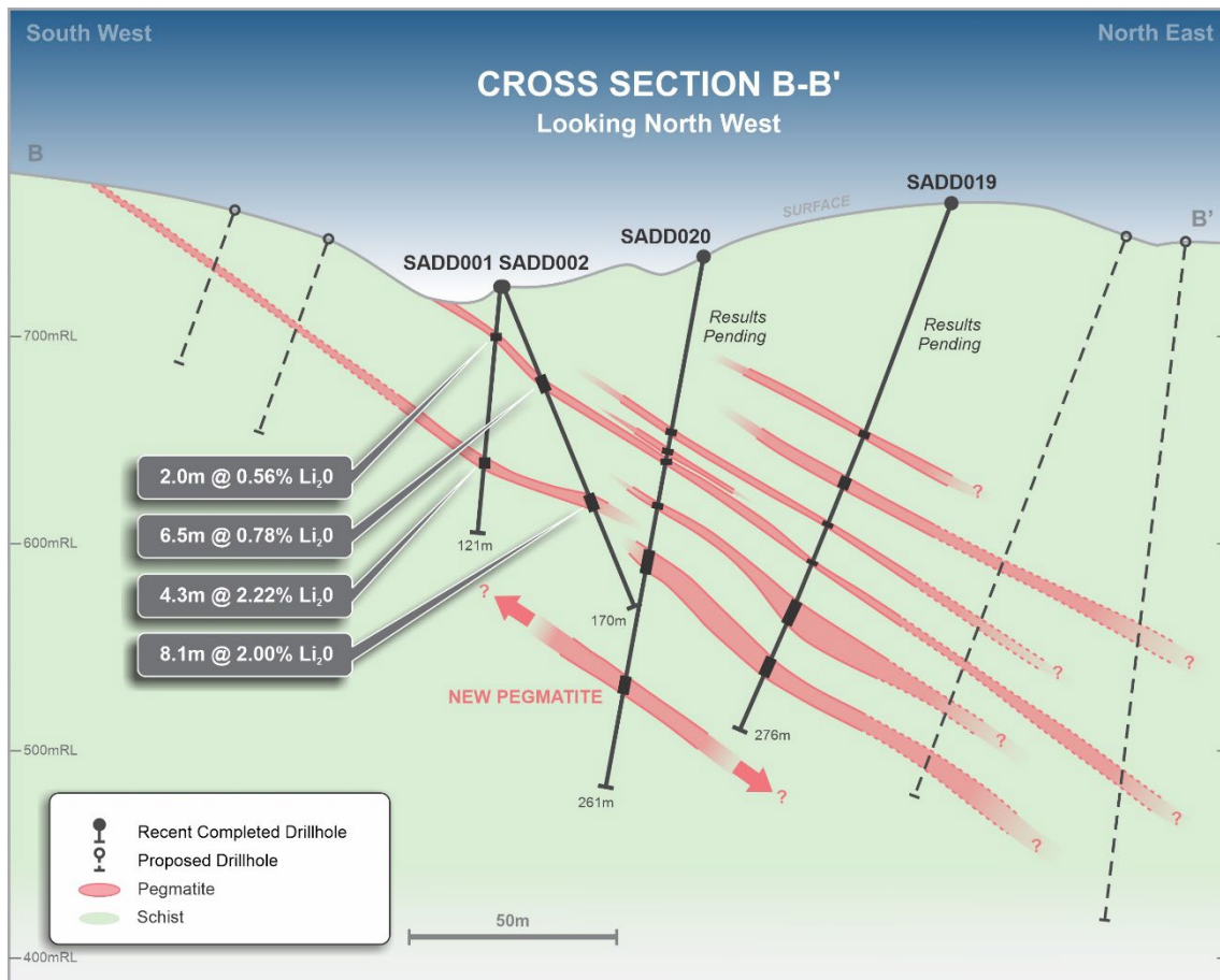
Figure 4: Drill section B-B1' showing completed and planned drill holes, and logged pegmatites for holes SADD019 and SADD020 (results pending) 6
