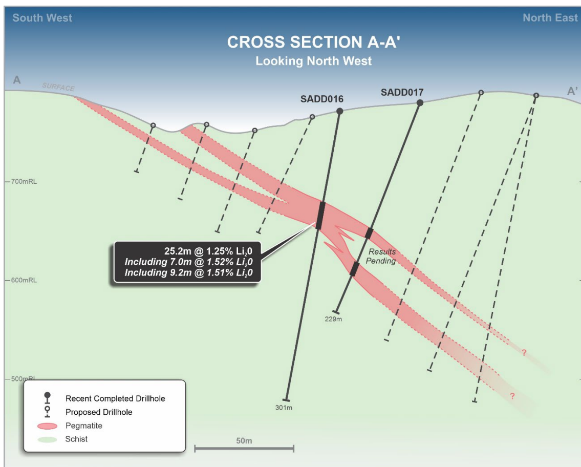
Figure 1: Drill section A-A' showing completed and planned drill holes, and results for SADD016 4 and logged pegmatite intersections for SADD017 (results pending)
