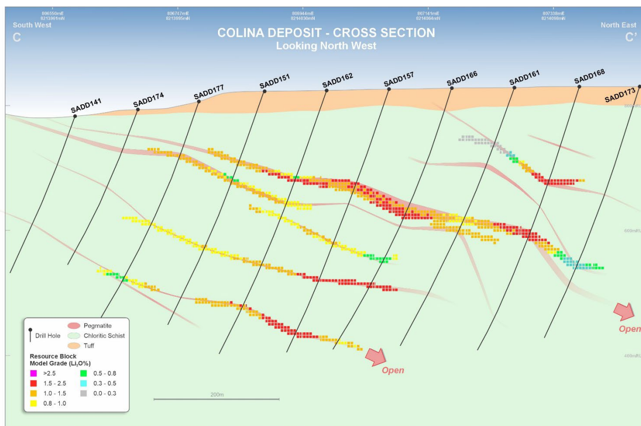
Figure 7: Colina MRE Block Model cross section 'C-C'.
