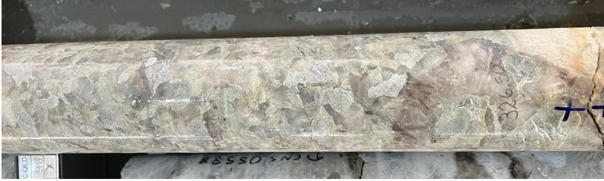
SADD246: ~326.50m (3.23% Li 2 O). Green spodumene associated to quartz, feldspar and mica.
