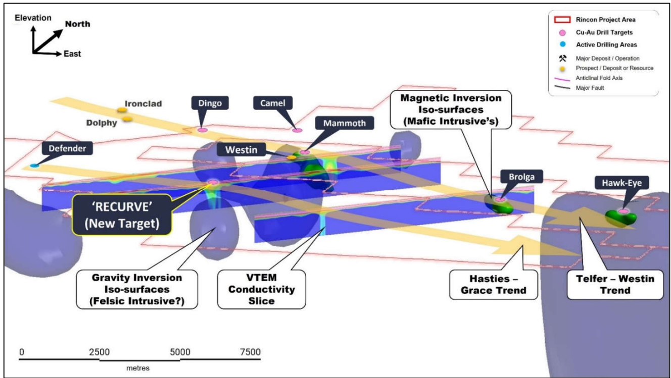
Figure 2: Isometric view looking to the northwest on the new 'Recurve' Au-Cu target showing 3D gravity inversion modelling results as low-density body iso-surfaces (blue), selected VTEM conductivity cross-section slices, 3D magnetic inversion modelling (green), mineralised trends and prospect prospects, and targets.
