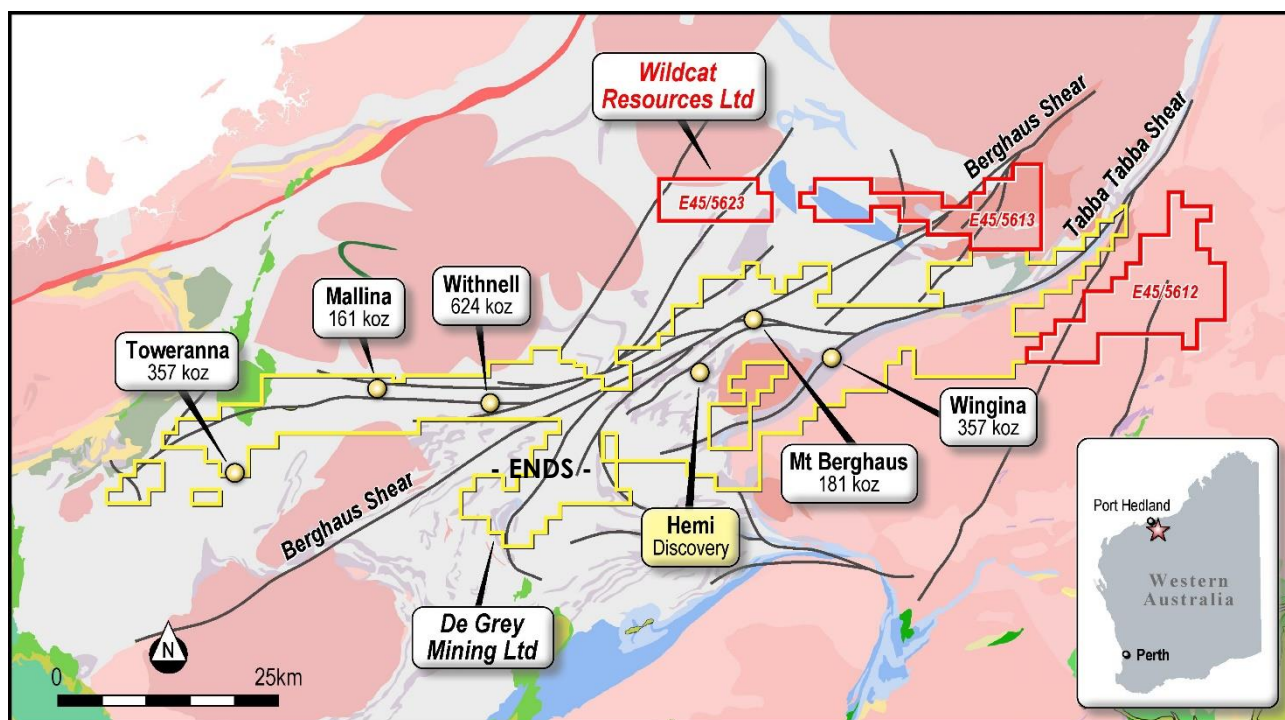
Figure 3 – Regional geological map of the Mallina Province - Pilbara Western Australia
