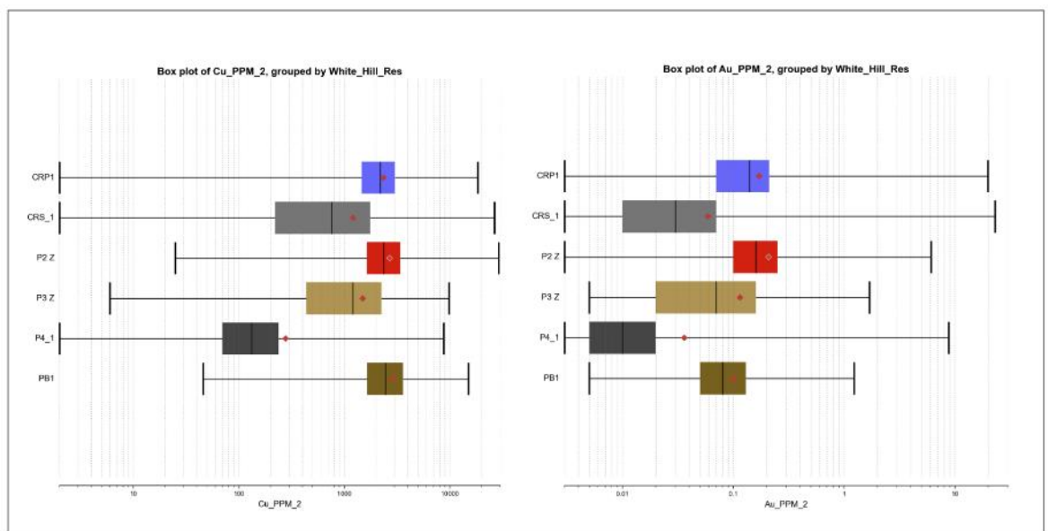
Figure 14-24: Box plot for raw Cu ppm and Au ppm data against group lithology (log scale)
