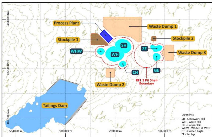
Figure 16-11: Site layout
