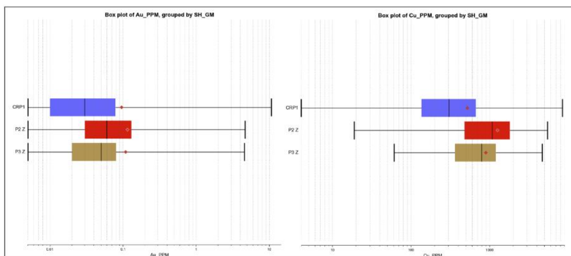
Figure 14-44: Box plot for raw Cu ppm and Au ppm data against group lithology (log scale) for Zephyr
