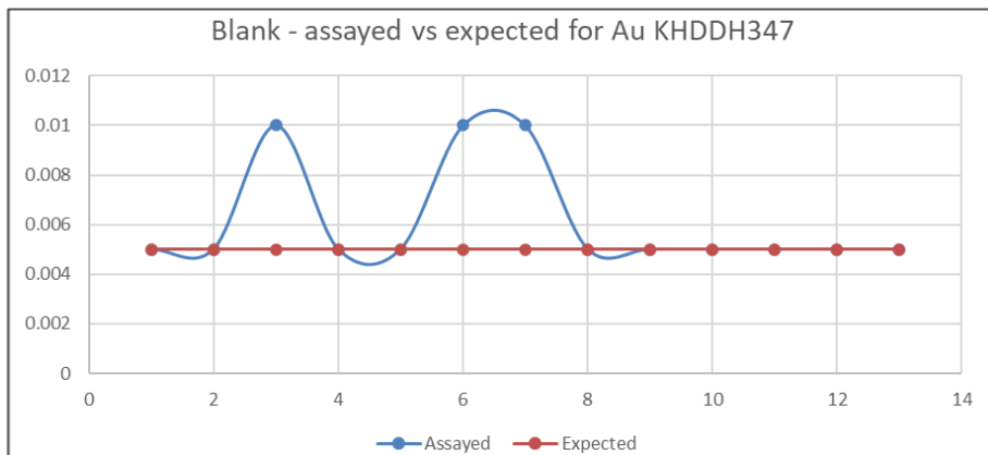
Figure 12-16: Performance chart of KHDDH347 Au umpire outcomes by ALS
