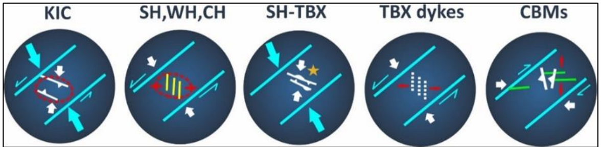
Figure 7-5: The structural framework for formation of mineralisation at Kharmagtai
