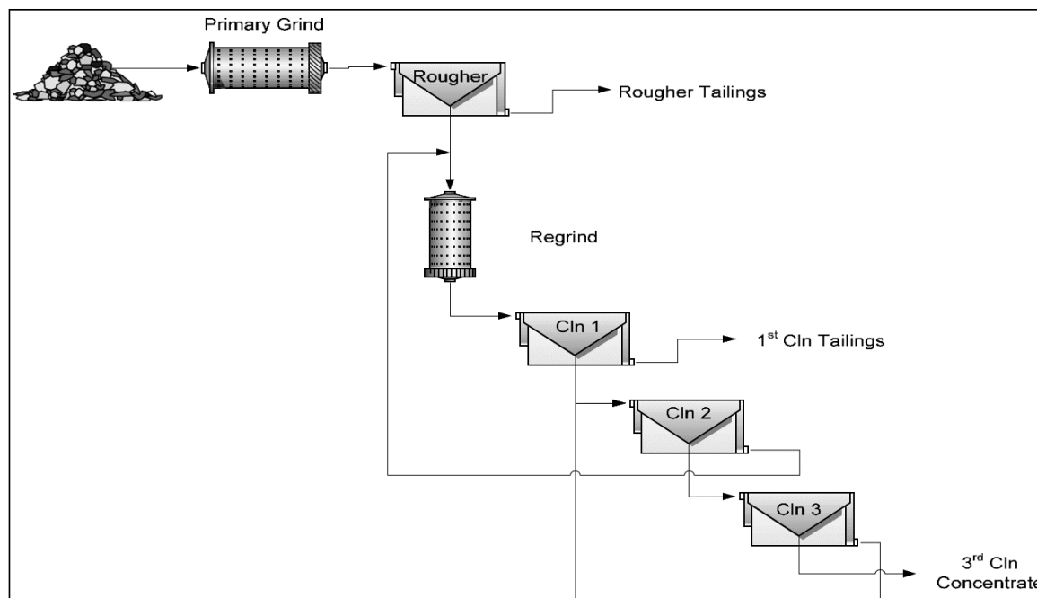
Figure 13-3: Process flowsheet
